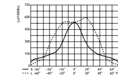
Iodure double culot 150 W L.O.R. = 0,76 • 1 x 12900 lm
